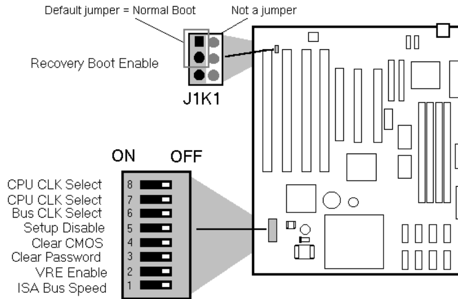
Figure B-1. Jumper locations and settings (default settings shown)
